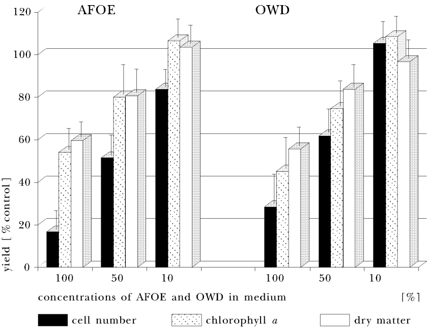
Fig. 1. Growth of the Scenedesmus armatus population exposed to No. II diesel fuel oil added to the culture medium in the form of aqueous fuel oil extract (AFOE) and oil-in-water dispersion (OWD) after 7 days of culture. AFOE and OWD, prepared from 50 and 1 cm 3 of oil in 1 dm 3 of medium, contain hydrocarbons at a concentration of 49.8 ppm and 15.1 ppm respectively. The vertical bars indicate the standard error of the mean
